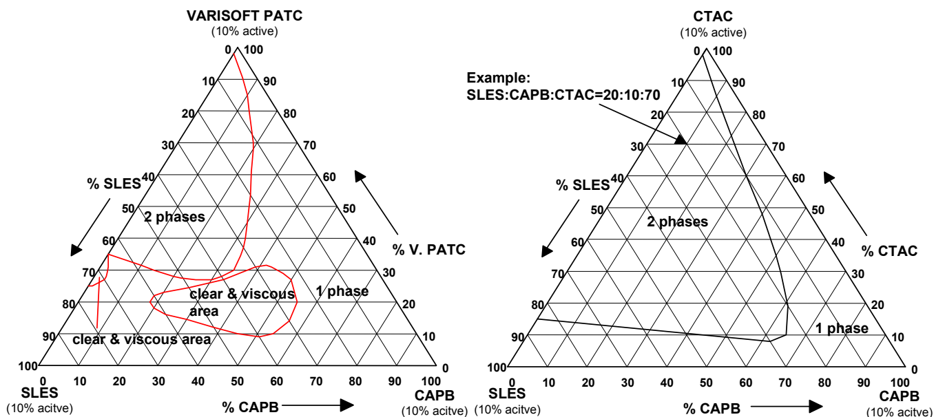
Figure 2: Phase diagrams of VARISOFT® PATC and Cetrimonium Chloride (VARISOFT® 300)
