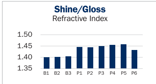
All Versagel SF blends have higher RI than all commercial hair oil product benchmarks.
